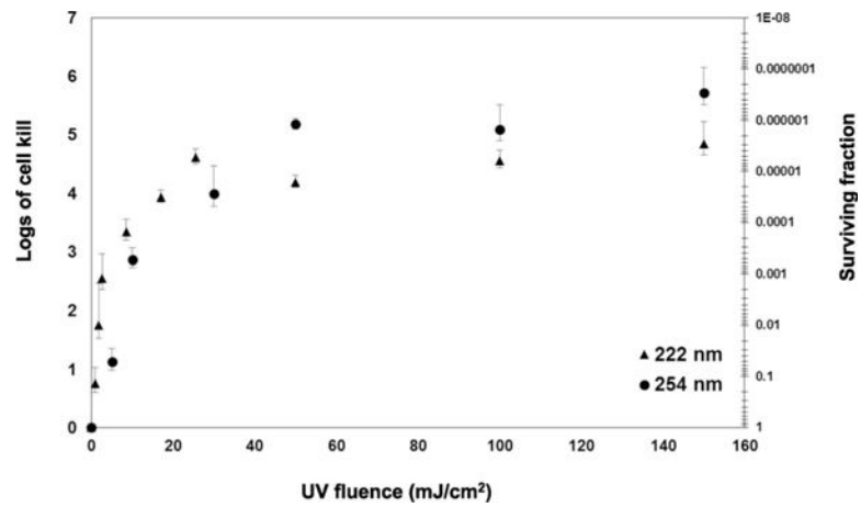
FIG. 2. Bacterial cell killing induced by 222- and 254-nm UV light. Killing of MRSA (strain USA300) is shown relative to zero-fluence controls, expressed as surviving fraction or as logs of cell kill ( -\log_{10}[\text{surviving fraction}] ), produced by different fluences of UV light from a filtered 222-nm Kr-Cl excimer lamp ( \blacktriangle ) or a germicidal 254-nm lamp ( \bullet ).
